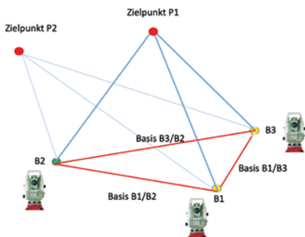
Abbildung 5-3: Triangulationsbasis
